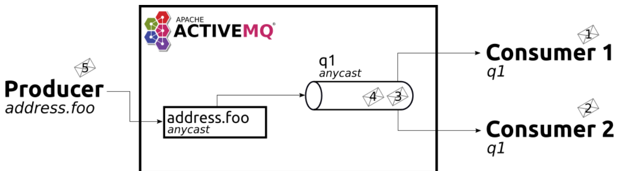
Figure 1. Anycast
