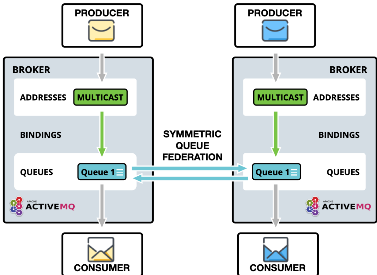
Figure 2. Queue Federation
