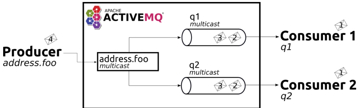
Figure 2. Multicast
