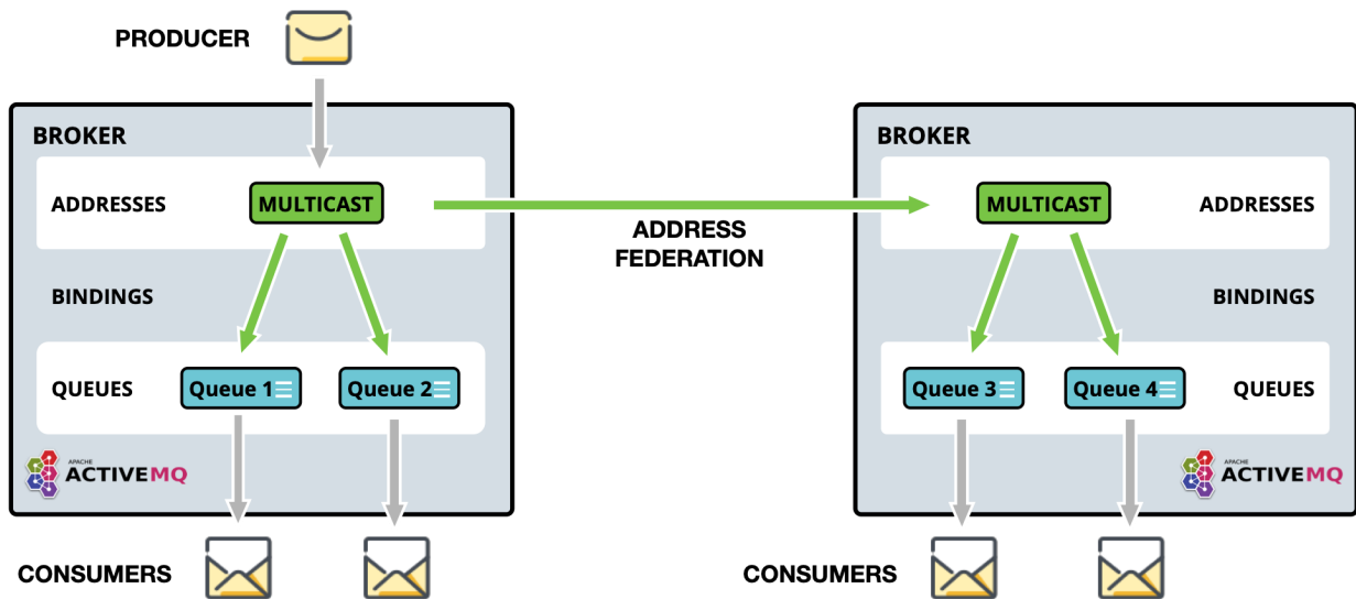
Figure 1. Address Federation
