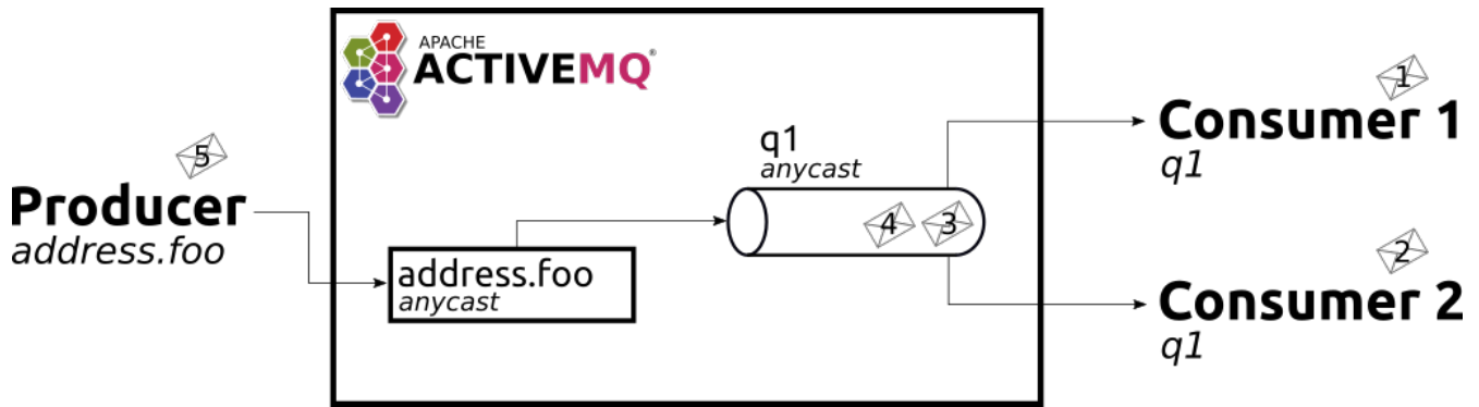
Figure 1. Anycast
