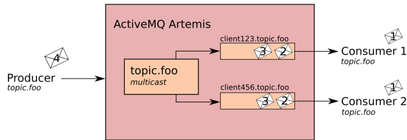
Figure 2. Publish-Subscribe
