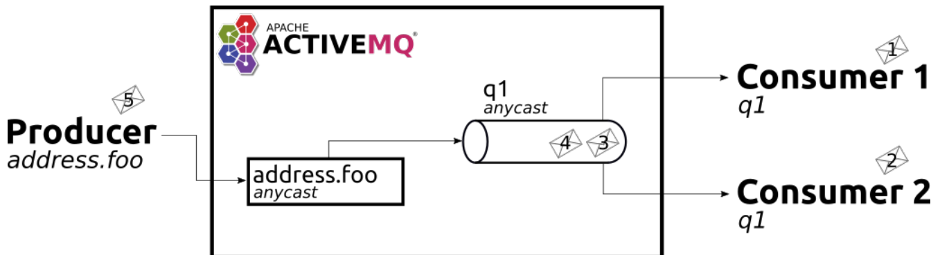
Figure 1. Anycast
