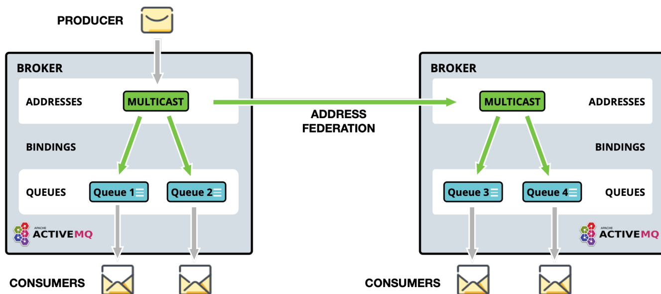
Figure 1. Address Federation
